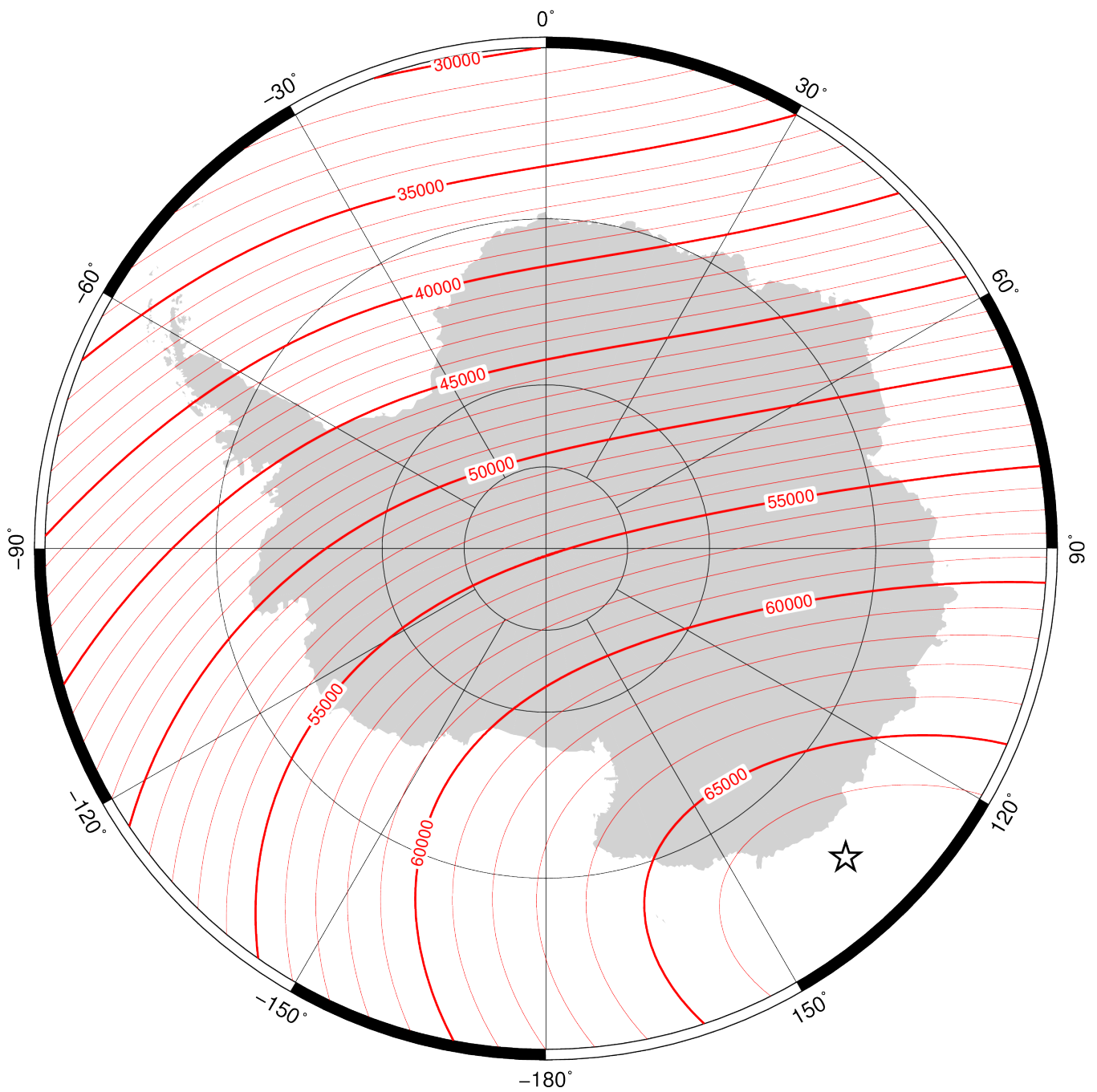
Total intensity ( F ) in region of south pole at 2020.0 from the World Magnetic Model (WMM2020). Contour interval is 1000 nT, white star is location of a magnetic pole and projection is Polar Stereographic. Credit: British Geological Survey (UK Research and Innovation).
