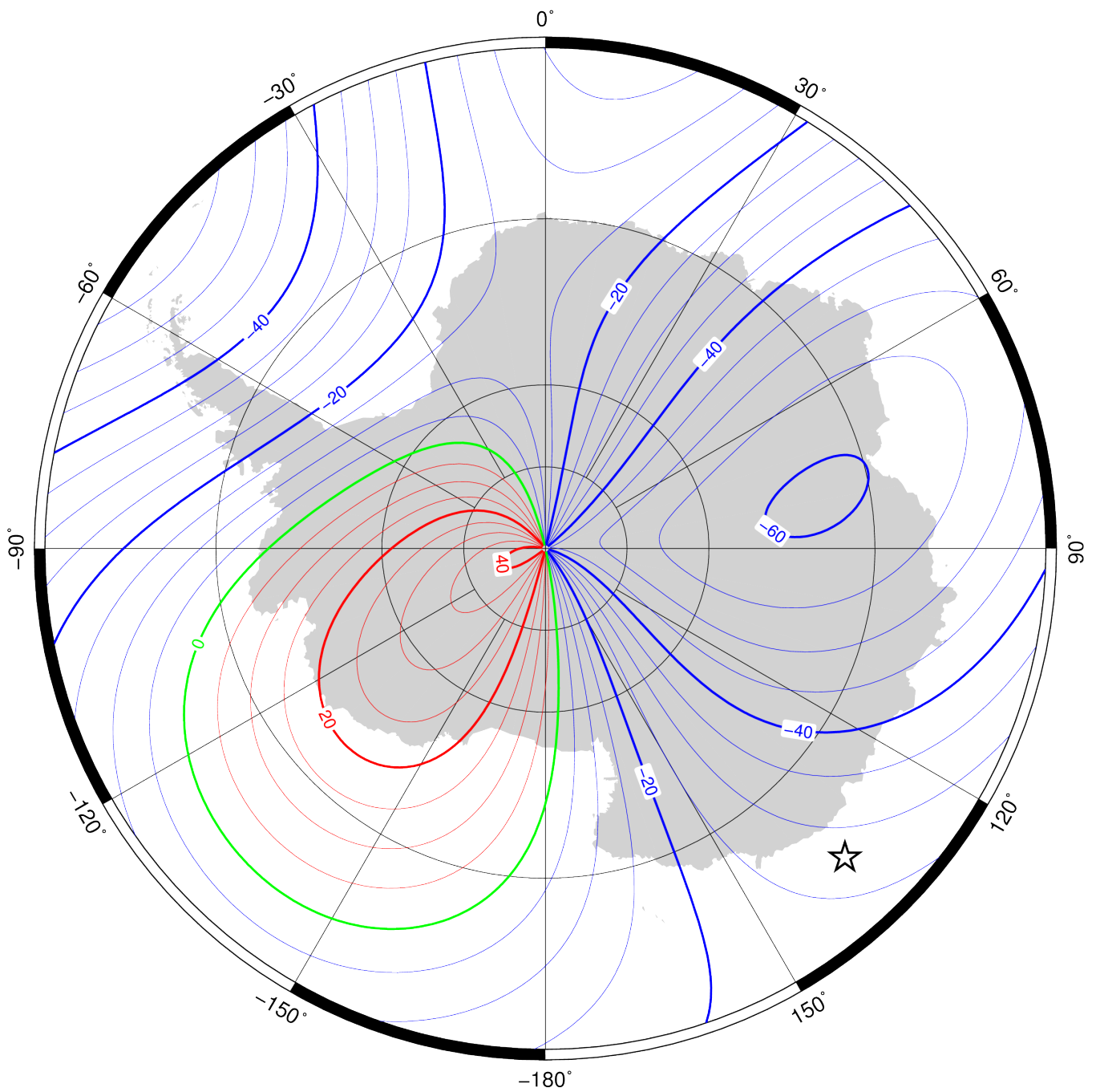
Annual rate of change of north component in region of south pole for 2020.0 to 2025.0 from the World Magnetic Model (WMM2020). Red – positive change, blue – negative change, green – zero change. Contour interval is 5 nT/year, white star is location of a magnetic pole and projection is Polar Stereographic. Credit: British Geological Survey (UK Research and Innovation).
