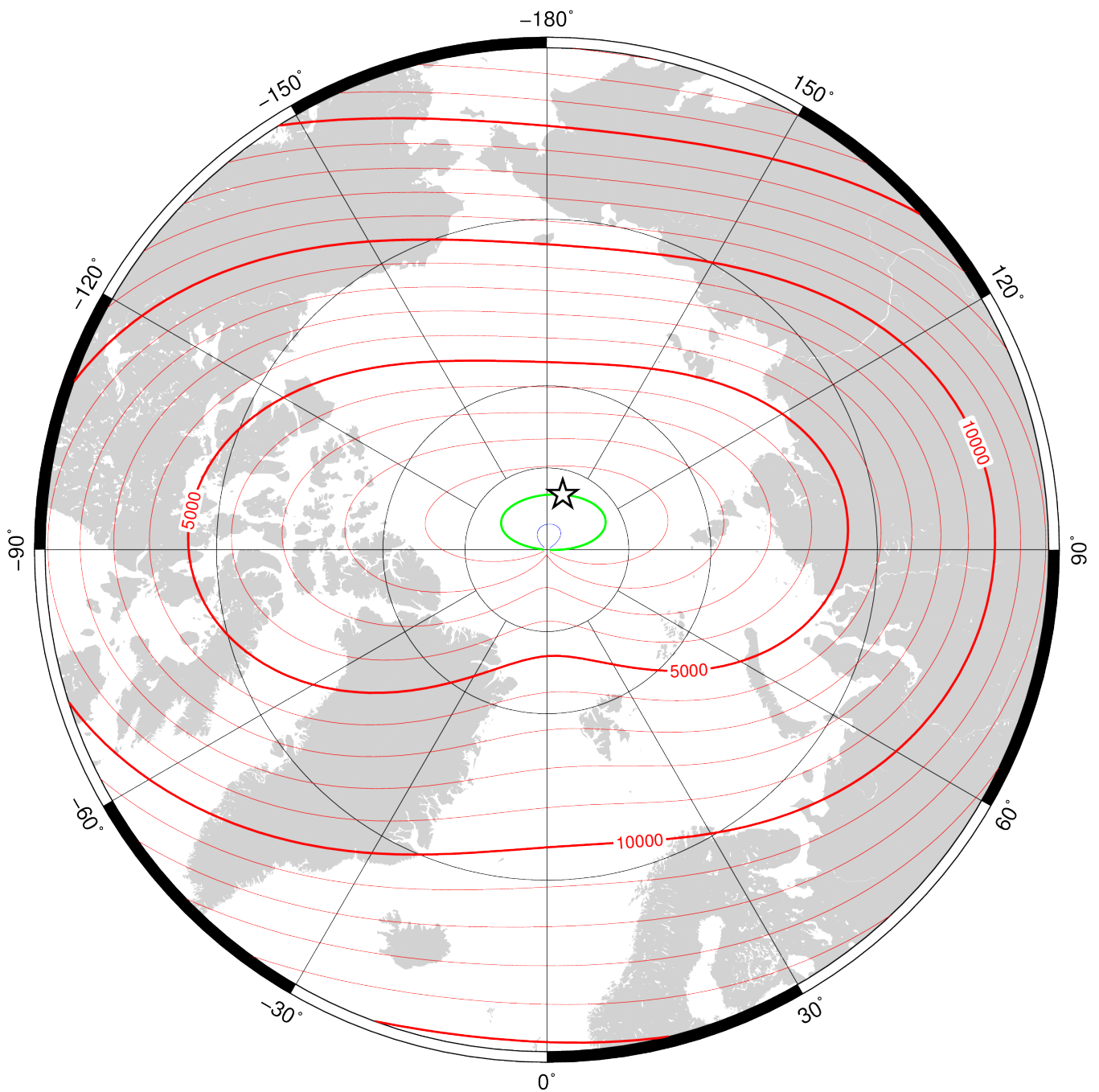
North component ( X ) in region of north pole at 2020.0 from the World Magnetic Model (WMM2020). Red – positive (north), blue – negative (south), green – zero. Contour interval is 1000 nT, white star is location of a magnetic pole and projection is Polar Stereographic. Credit: British Geological Survey (UK Research and Innovation).
