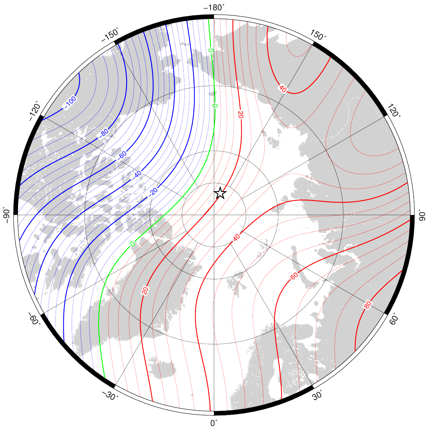
Annual rate of change of vertical component in region of north pole for 2020.0 to 2025.0 from the World Magnetic Model (WMM2020). Red – positive change, blue – negative change, green – zero change. Contour interval is 5 nT/year, white star is location of a magnetic pole and projection is Polar Stereographic. Credit: British Geological Survey (UK Research and Innovation).
