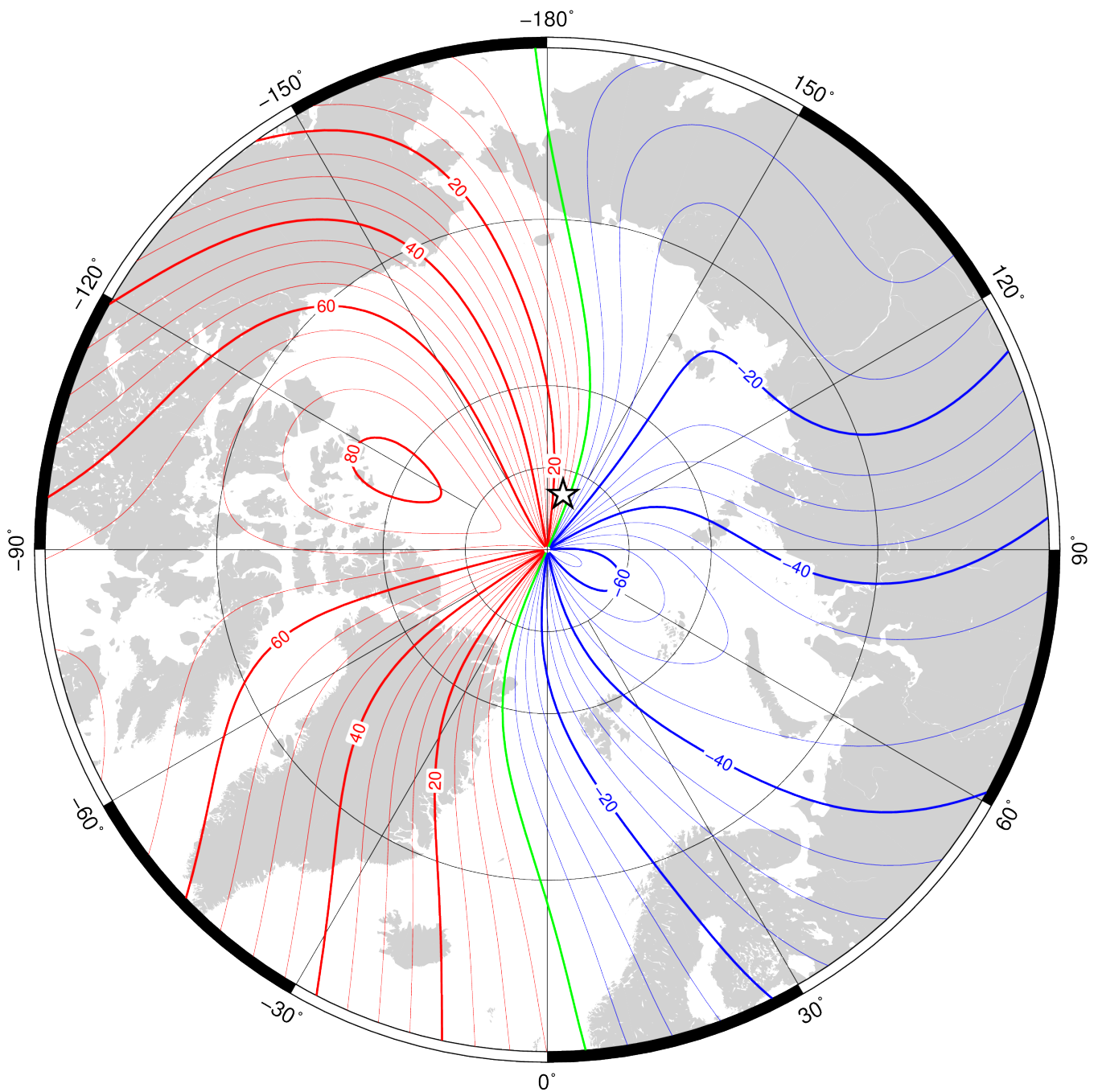
Annual rate of change of north component in region of north pole for 2020.0 to 2025.0 from the World Magnetic Model (WMM2020). Red – positive change, blue – negative change, green – zero change. Contour interval is 5 nT/year, white star is location of a magnetic pole and projection is Polar Stereographic. Credit: British Geological Survey (UK Research and Innovation).
