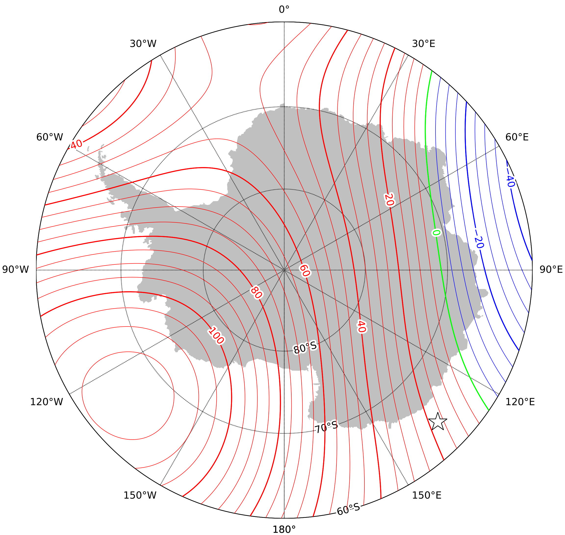
Annual rate of change of downward component in the region of the south pole at 2027.5 from the World Magnetic Model (WMM) 2025. Red - positive (downward) change, blue - negative (upward) change, green - zero change. Contour interval is 5nT/year, white star is the location of a magnetic pole and the projection is Polar Stereographic. This is an example of an isoporic chart. British Geological Survey © UKRI 2024
