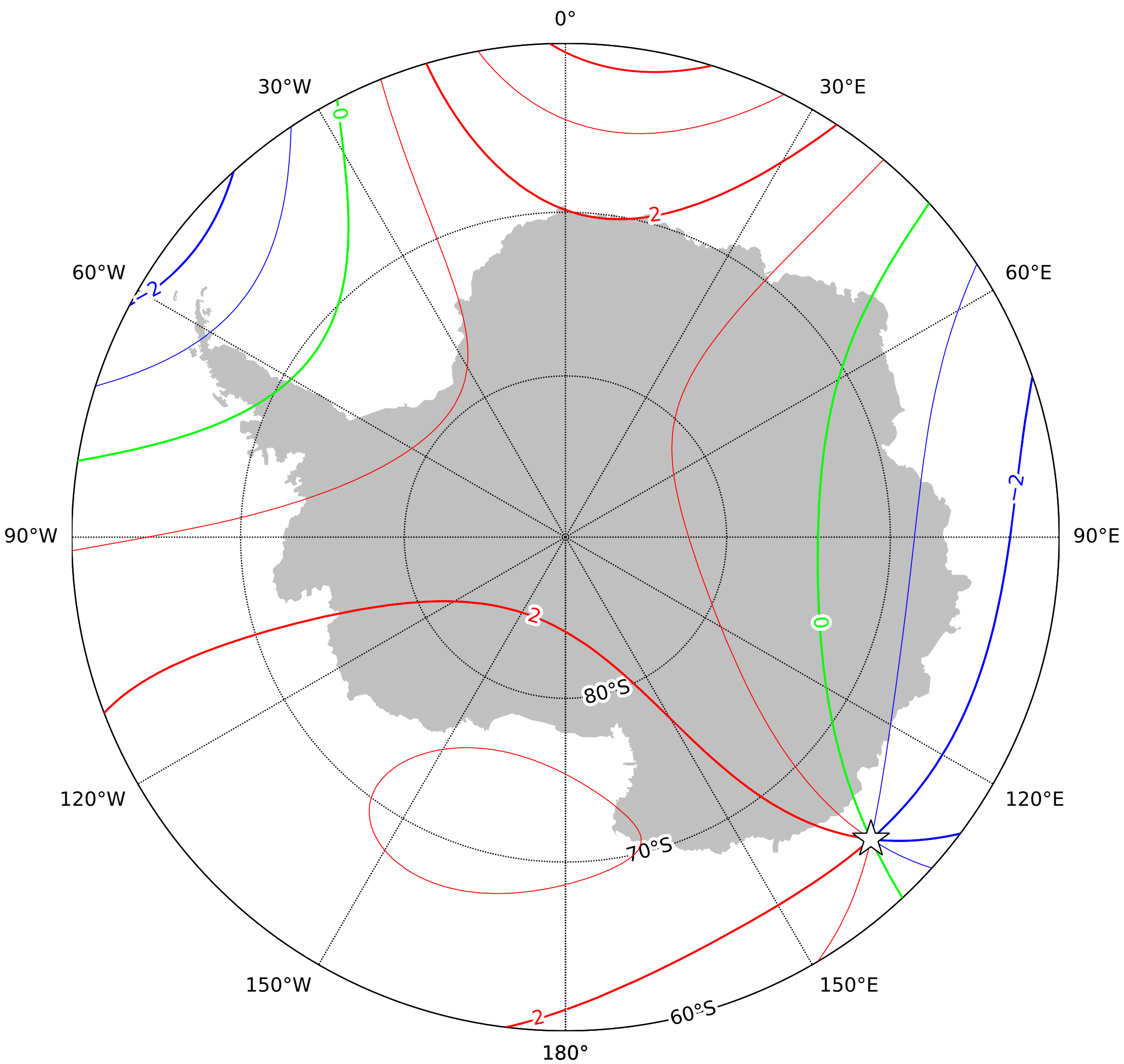
Annual rate of change of inclination in the region of the south pole at 2027.5 from the World Magnetic Model (WMM) 2025. Red - positive (downward) change, blue - negative (upward) change, green - zero change. Contour interval is 1'/year, white star is the location of a magnetic pole and the projection is Polar Stereographic. This is an example of an isoporic chart. British Geological Survey © UKRI 2024
