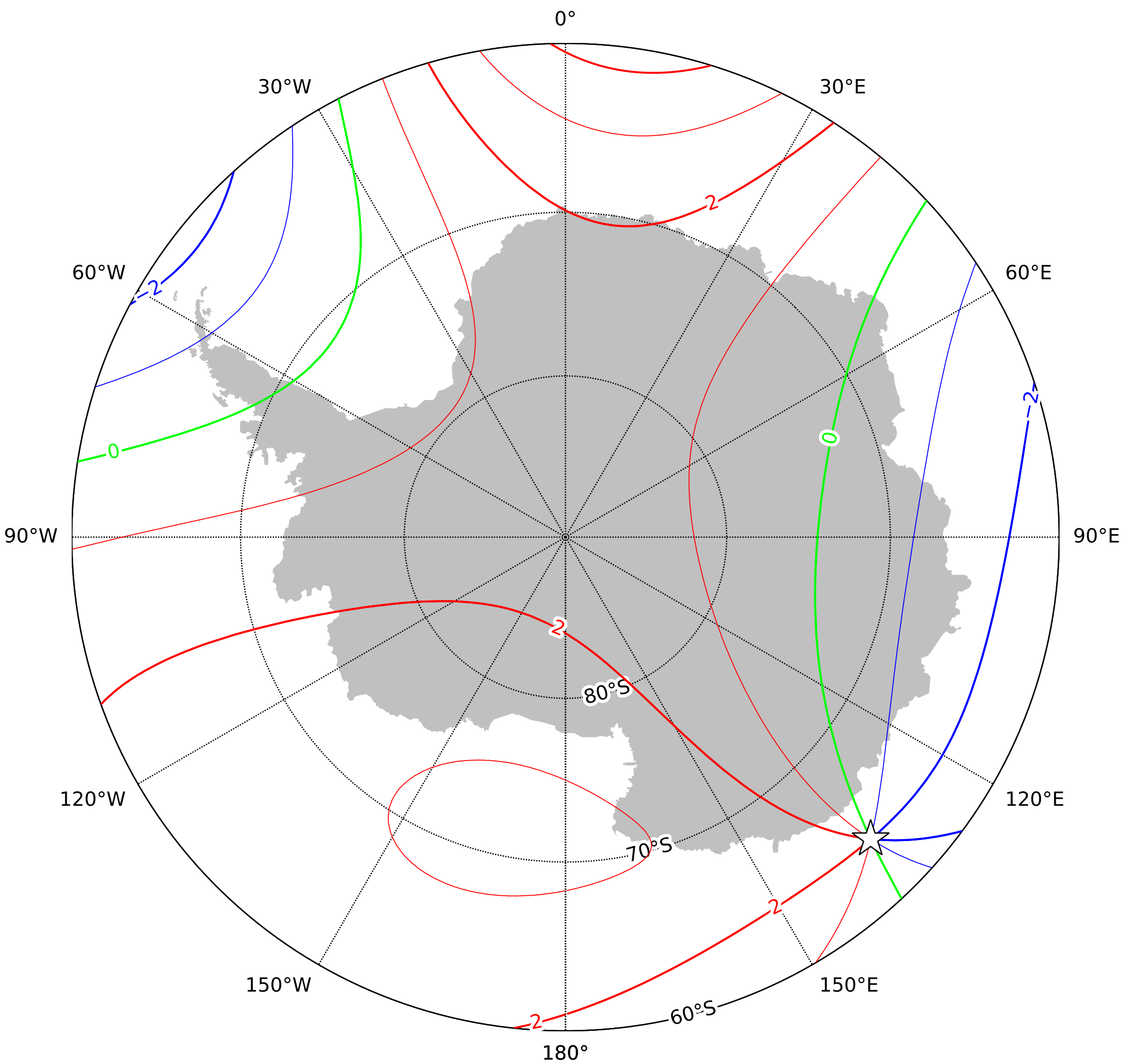
Annual rate of change of inclination in the region of the south pole at 2027.5 from the World Magnetic Model - High Resolution (WMMHR) 2025 (core component only). Red - positive (downward) change, blue - negative (upward) change, green - zero change. Contour interval is 1'/year, white star is the location of a magnetic pole and the projection is Polar Stereographic. This is an example of an isoporic chart. British Geological Survey © UKRI 2024
