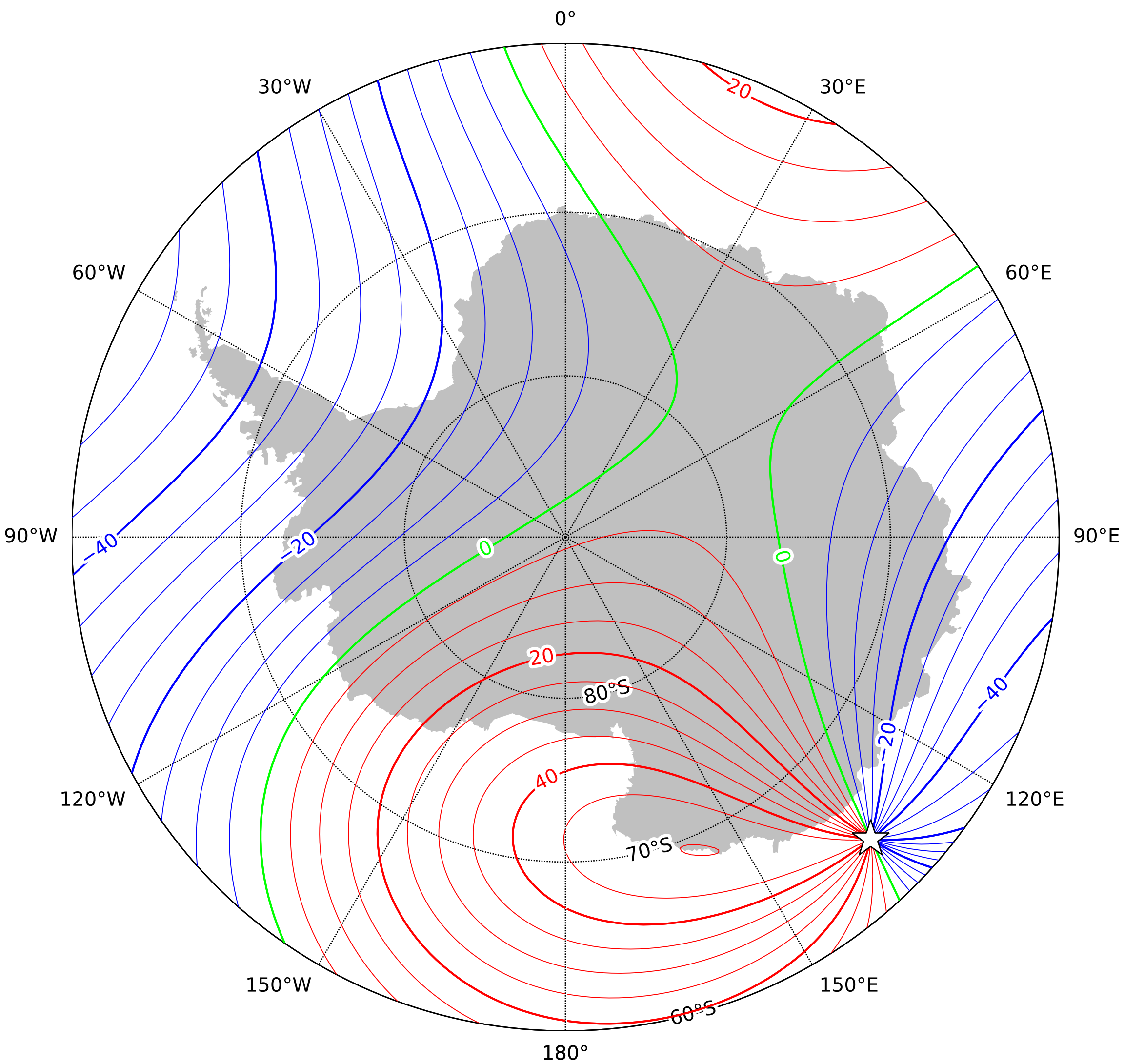
Annual rate of change of horizontal intensity in the region of the south pole at 2027.5 from the World Magnetic Model - High Resolution (WMMHR) 2025 (core component only). Red - positive change, blue - negative change, green - zero change. Contour interval is 5nT/year, white star is the location of a magnetic pole and the projection is Polar Stereographic. This is an example of an isoporic chart. British Geological Survey © UKRI 2024
