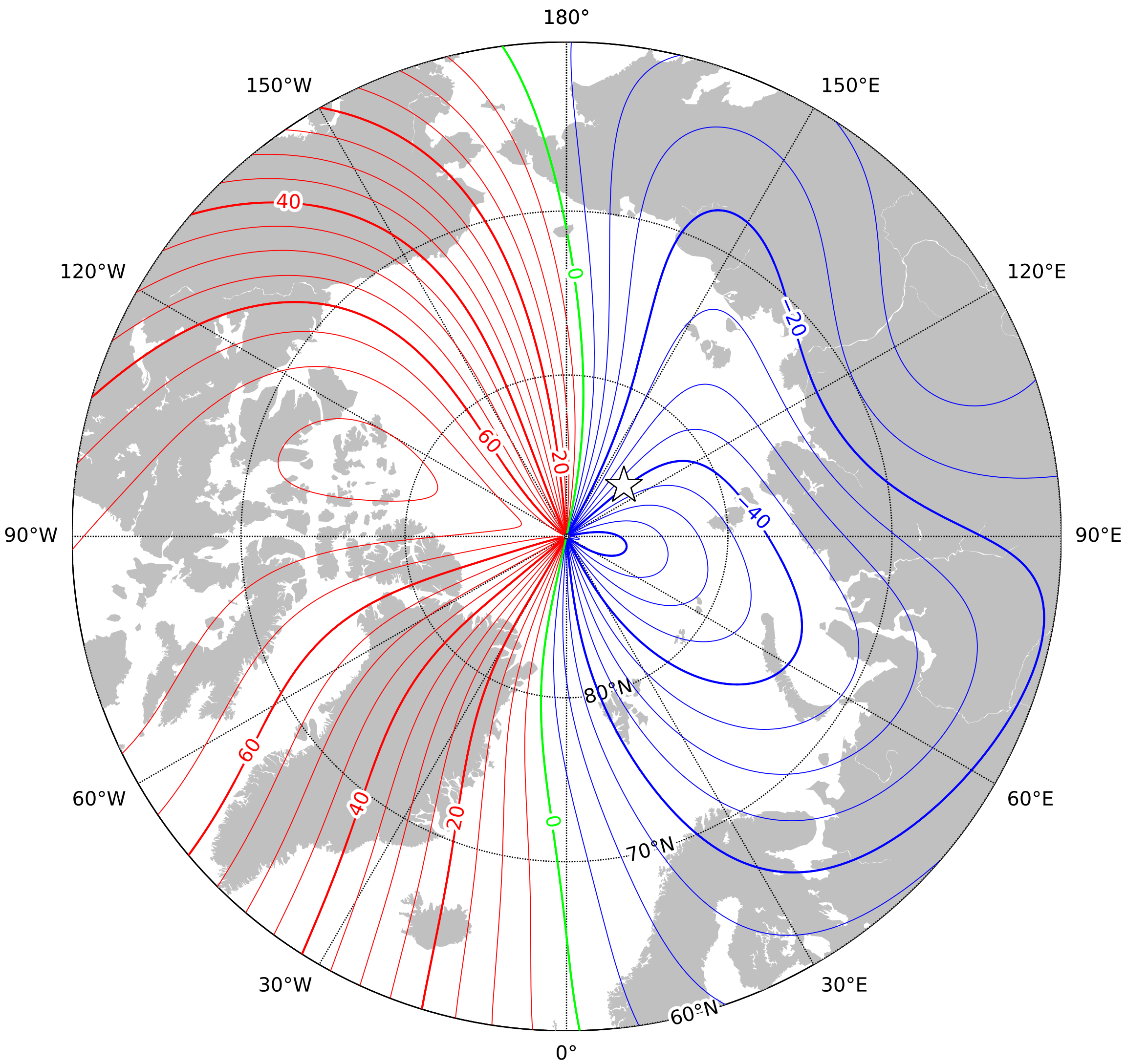
Annual rate of change of north component in the region of the north pole at 2027.5 from the World Magnetic Model - High Resolution (WMMHR) 2025 (core component only). Red - positive (northerly) change, blue - negative (southerly) change, green - zero change. Contour interval is 5nT/year, white star is the location of a magnetic pole and the projection is Polar Stereographic. This is an example of an isoporic chart. British Geological Survey © UKRI 2024
