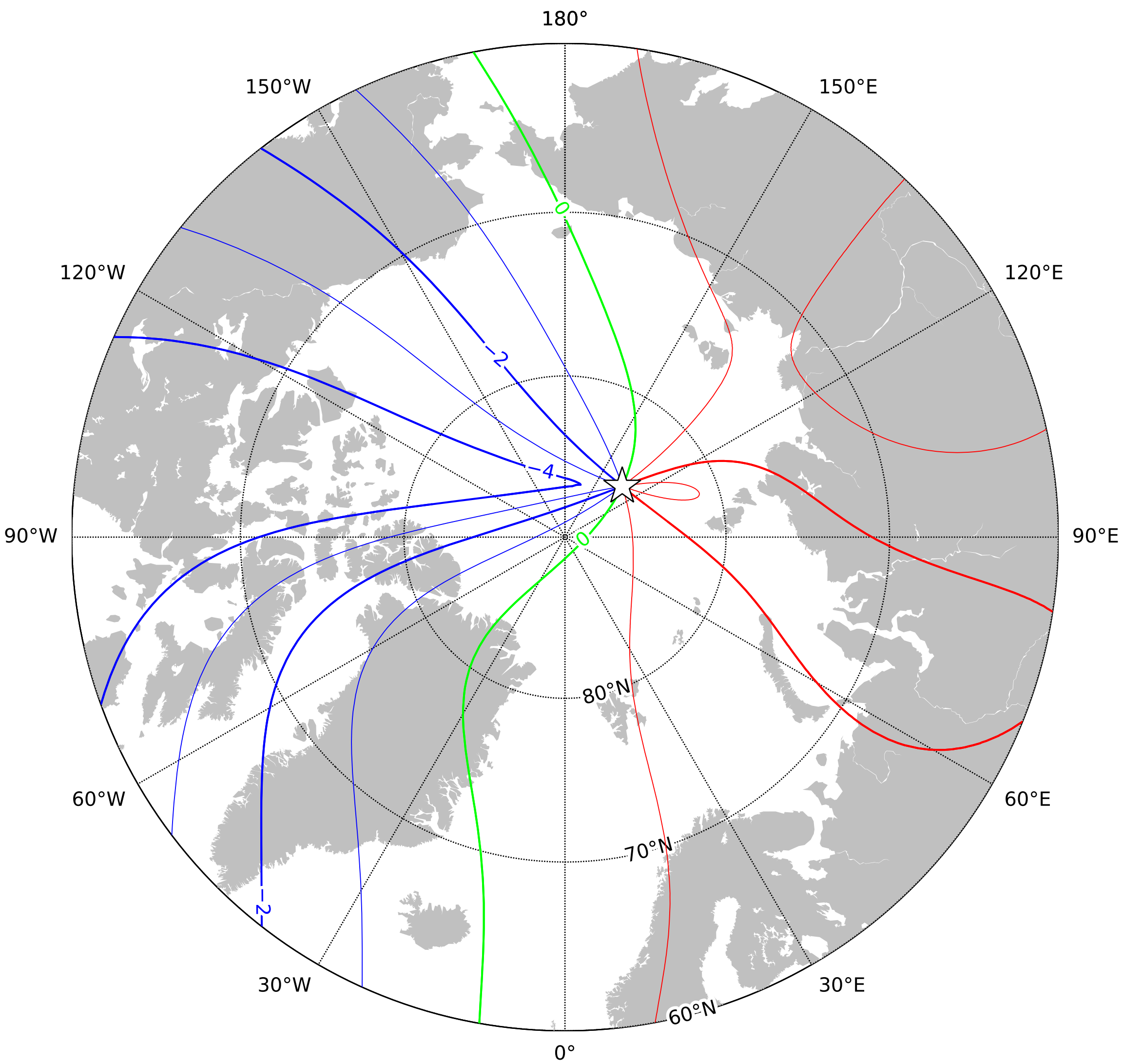
Annual rate of change of inclination in the region of the north pole at 2027.5 from the World Magnetic Model - High Resolution (WMMHR) 2025 (core component only). Red - positive (downward) change, blue - negative (upward) change, green - zero change. Contour interval is 1'/year, white star is the location of a magnetic pole and the projection is Polar Stereographic. This is an example of an isoporic chart. British Geological Survey © UKRI 2024
