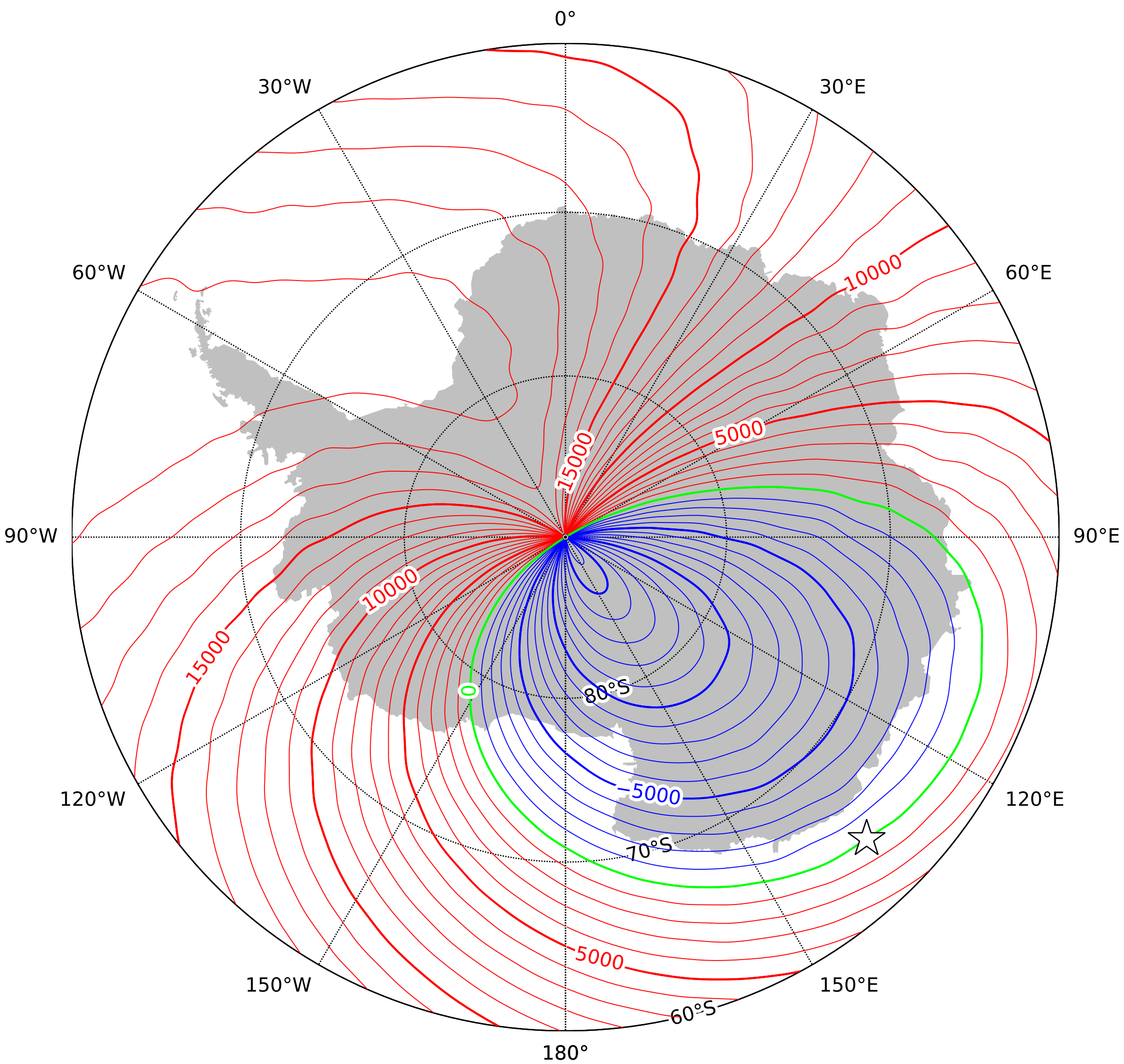
North component (X) in the region of the south pole at 2025.0 from the World Magnetic Model - High Resolution (WMMHR) 2025. Red - positive (north), blue - negative (south), green - zero. Contour interval is 1000nT, white star is the location of a magnetic pole and the projection is Polar Stereographic. This is an example of an isodynamic chart.
