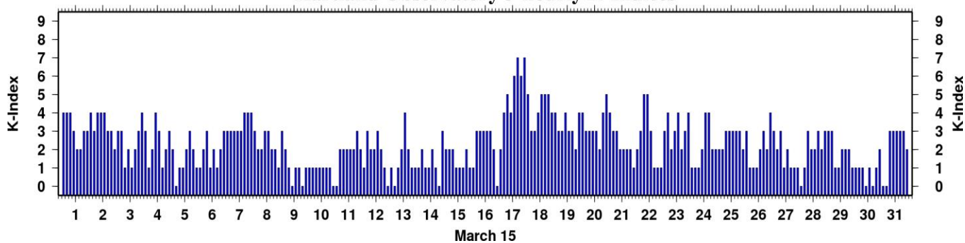
Hartland Observatory 3-hourly K-Indices
